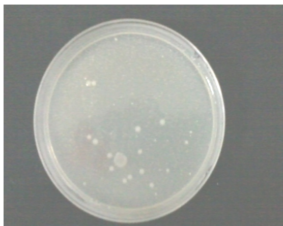
Fig 3: Representative of Ames spot test showing spontaneous His + revertants presence of sodium azide. The mean number of revertants observed from the open CFU was 88.67 colonies.
